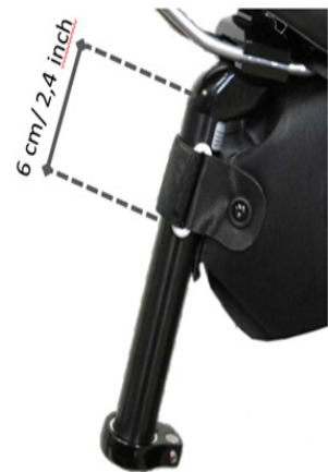
Space required for mounting Seat-Pack 11 L to the seat post
